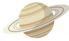
SATURN
