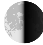
Last Quarter
