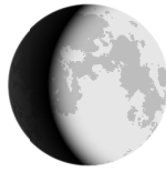
Waxing Gibbous
