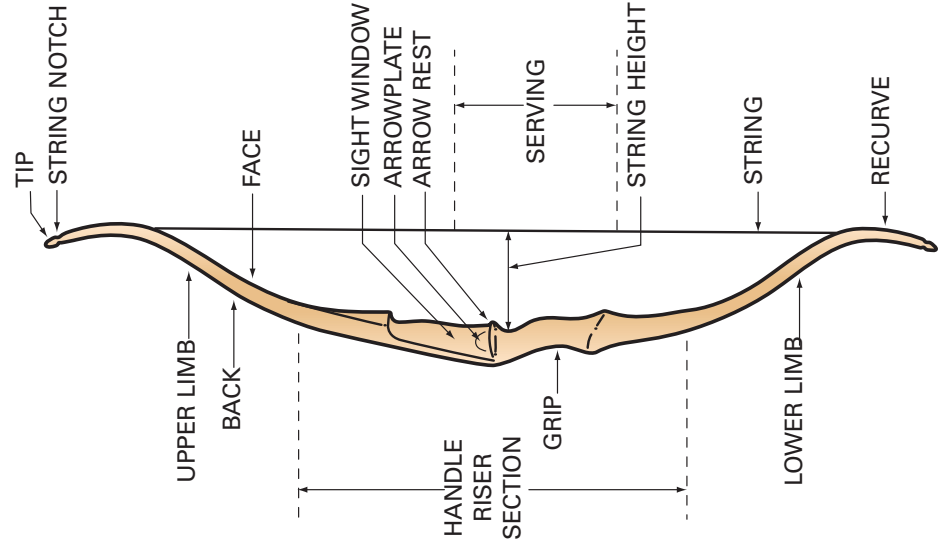
RECURVE BOW
