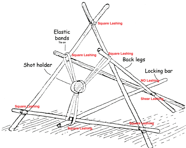
Catapult shown above made with BSA Scout hiking staff.
